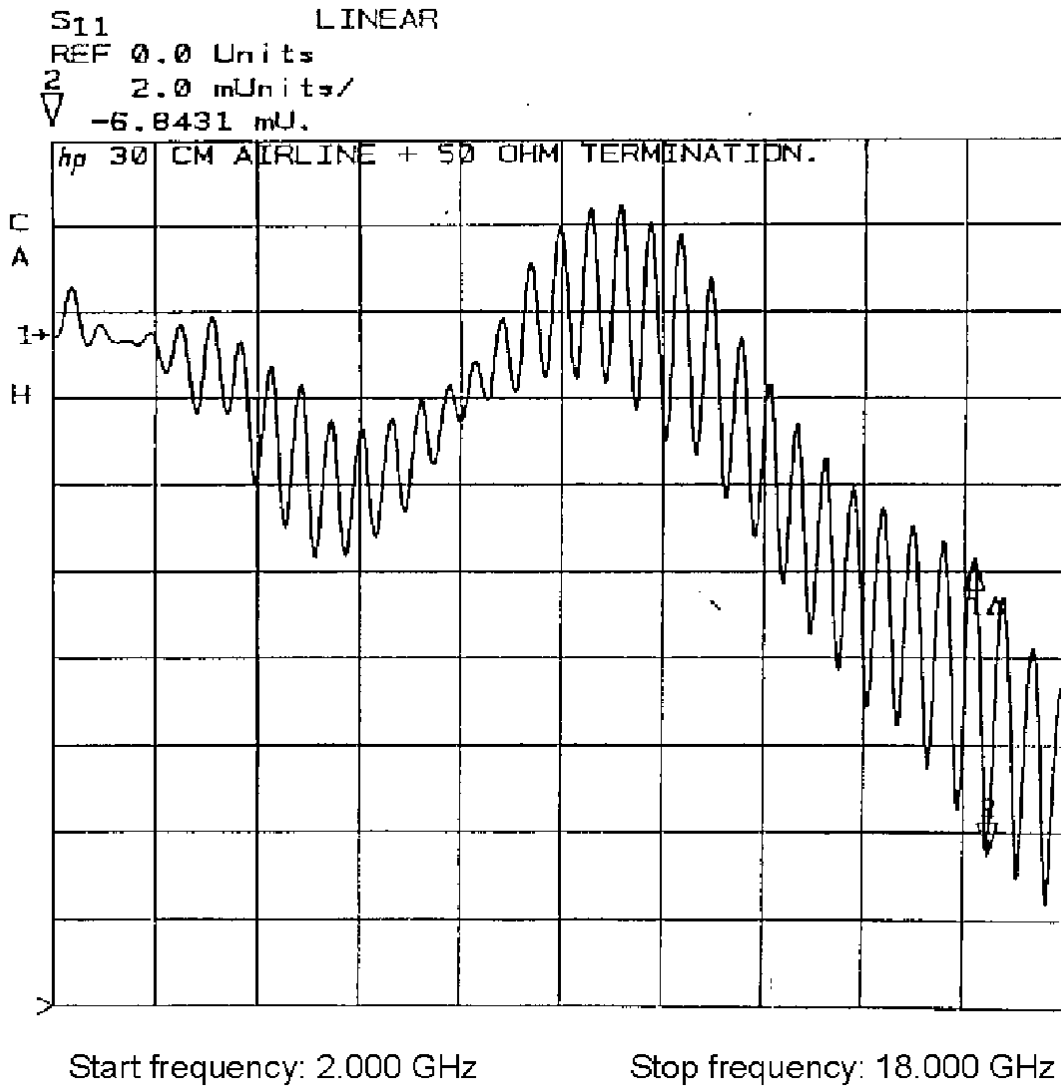
Figure 1: A non-perfect 50 Ω load is connected to a 30 cm airline. The other side of the airline is attached to port 1. This figure shows which kind of typical response will be obtained measuring S_{11} as function of frequency. From the ripple an effective directivity can be determined.
